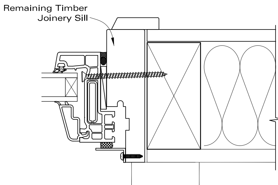
COVER JAMB FLASHING OPTION
