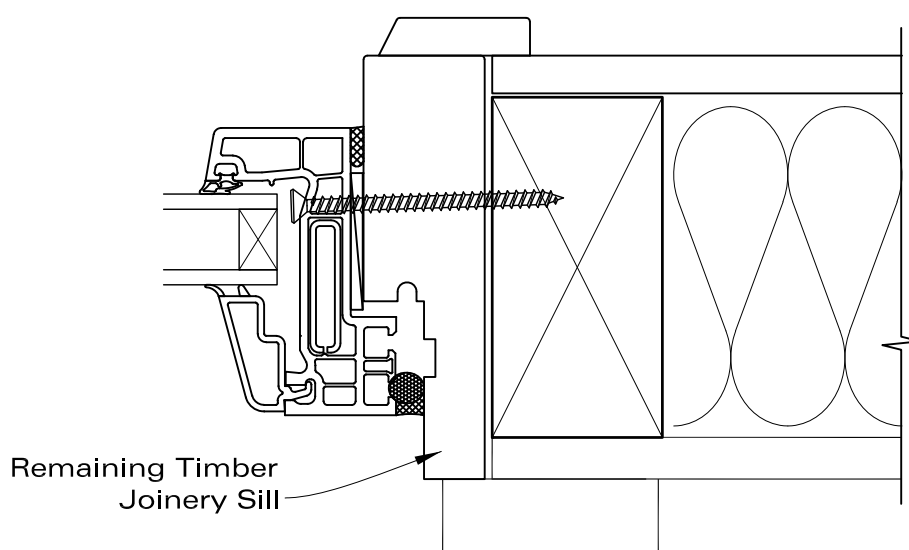
SEALANT OPTION
