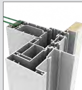
Sliding door jamb section.
