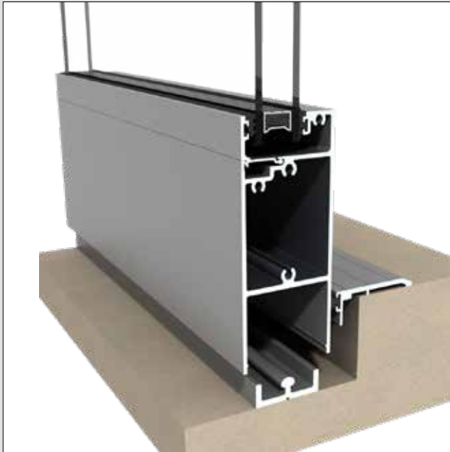
Magnum slider – stepped threshold shown.
