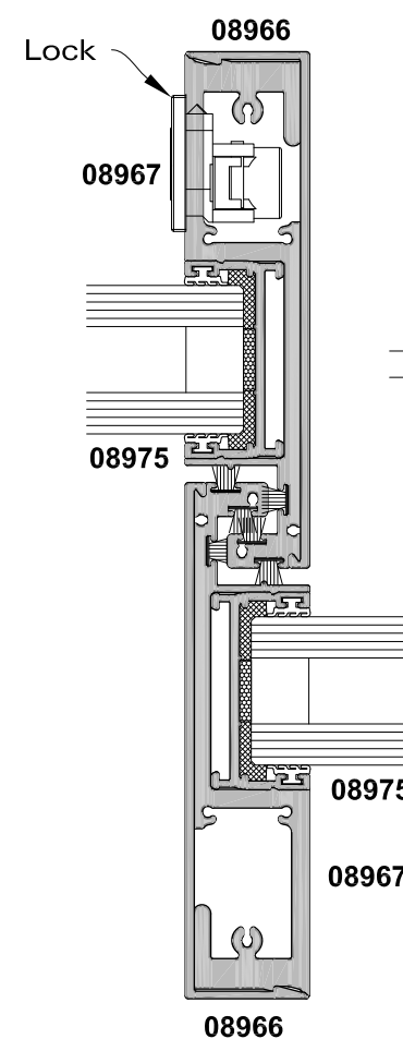
FIXED PANEL
