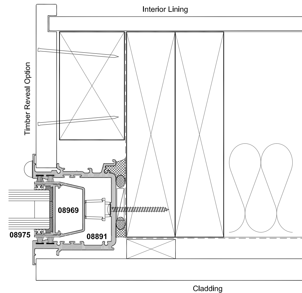
FIXED PANEL
