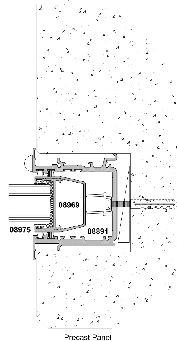
FIXED PANEL
