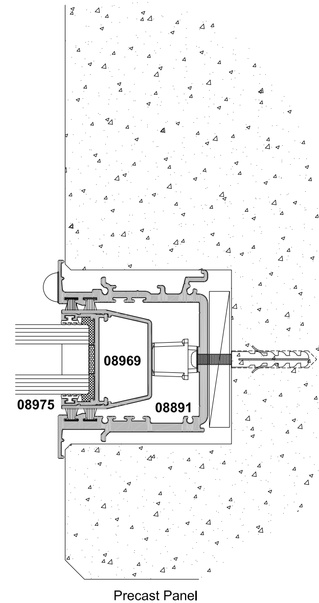
FIXED PANEL
