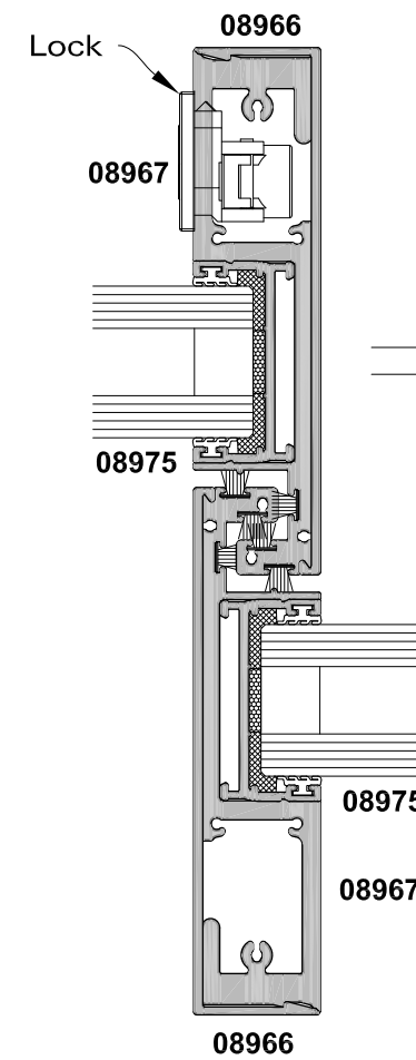
FIXED PANEL
