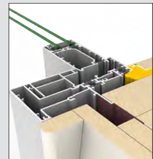
Sliding window jamb detail.
