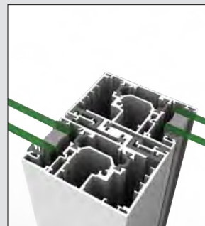
Fully thermally isolated interlocker stiles, shown in flush closed position.
