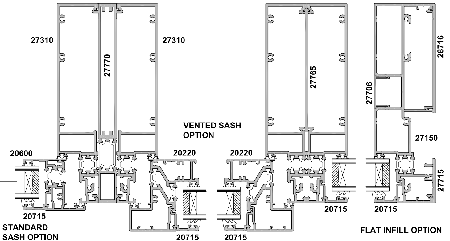
BOXED COUPLER MULLION OPTION
