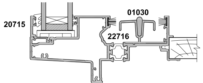
22050 PROJECTING FRAME OPTION
