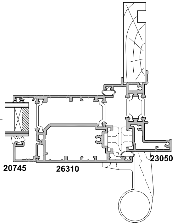
9260021 83mm Throw Hinge Option
