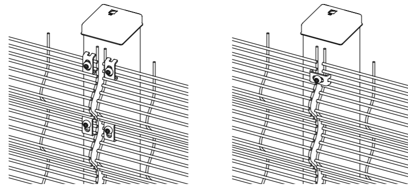
Fixing Detail
