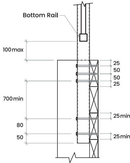
Steel Post: PBS-2.4-5CTR-GPCB or PBS-2.4-5CTR-GPC
