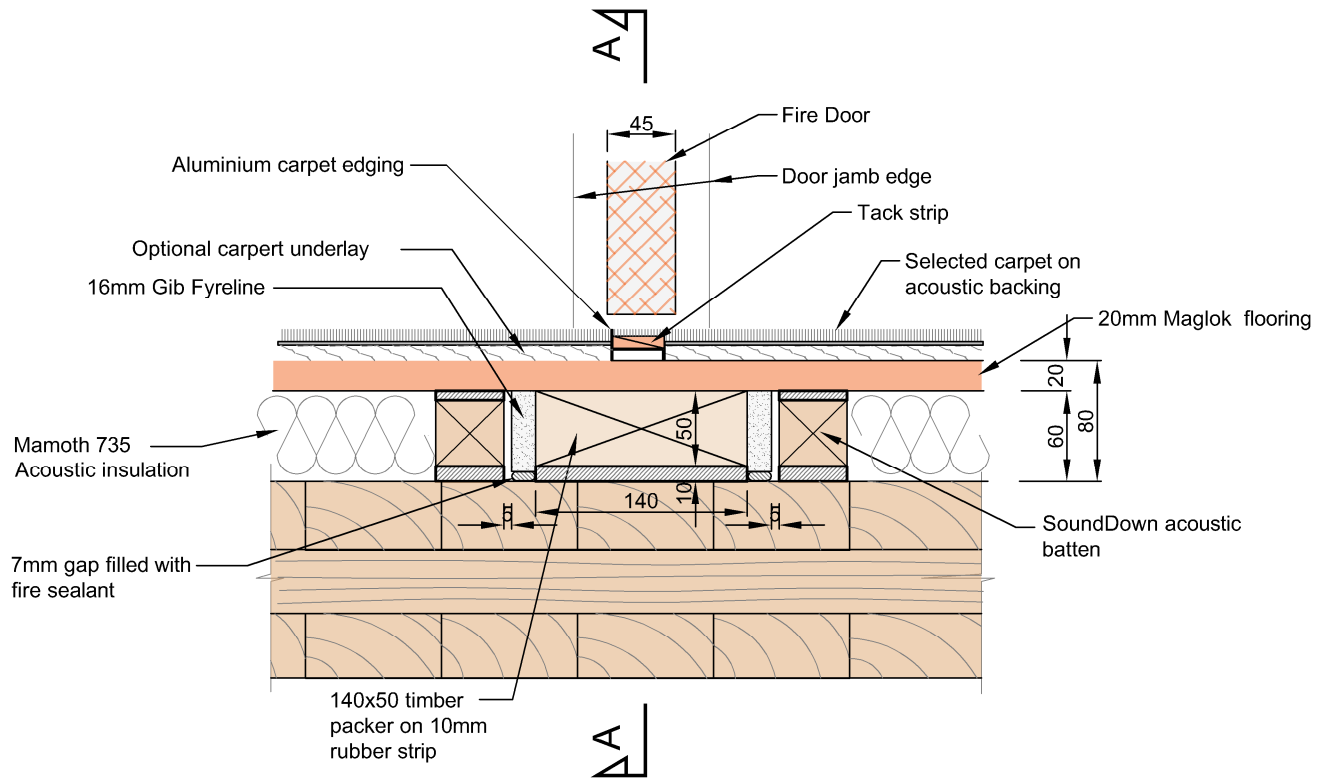
Floor System at Fire Door Maglok flooring Detail
