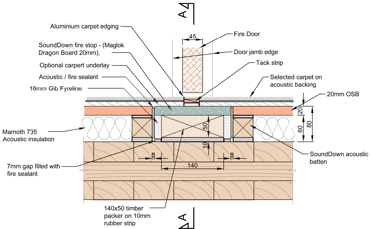
Floor System at Fire Door OSB Detail
