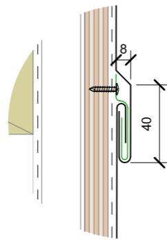
Euro Wall Lock Seam horizontal
