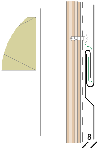
Euro Wall Flat Lock Horizontal
