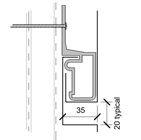
Euro Wall Flat Panel System horizontal
