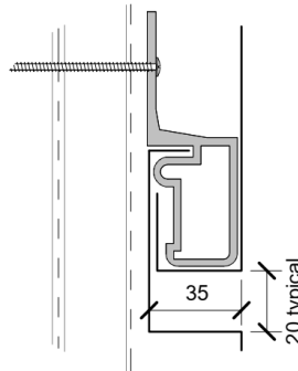
Euro Wall Flat Panel System horizontal
