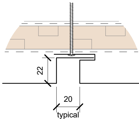
Euro Wall Cassette vertical
