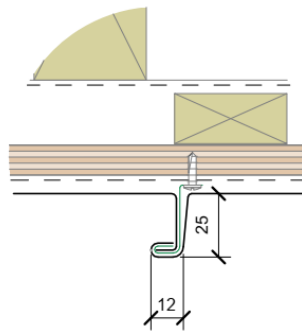
Euro Wall Angle Seam 25 vertical
