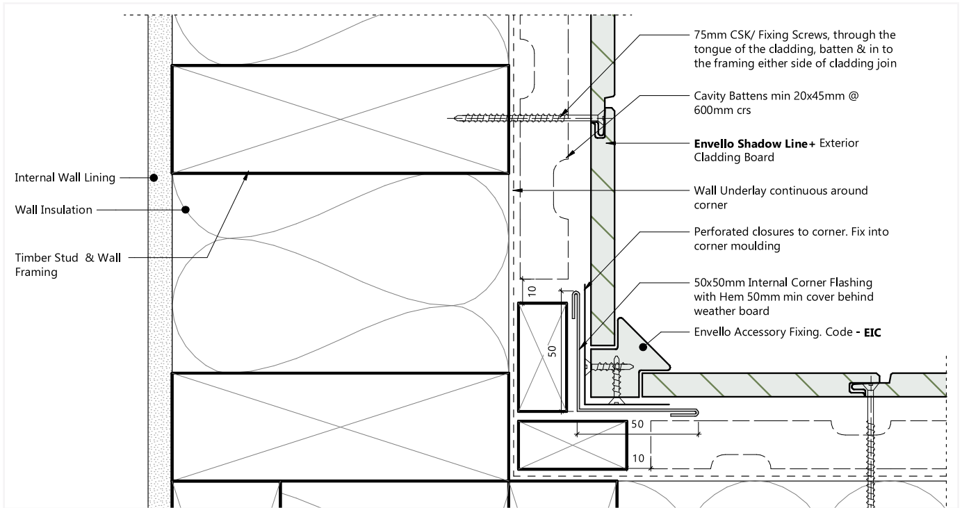
FIG. 9 - INTERNAL CORNER PROFILE
