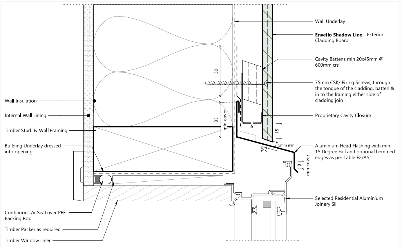
FIG. 5 - BATTEN LAYOUT BELOW A SILL
