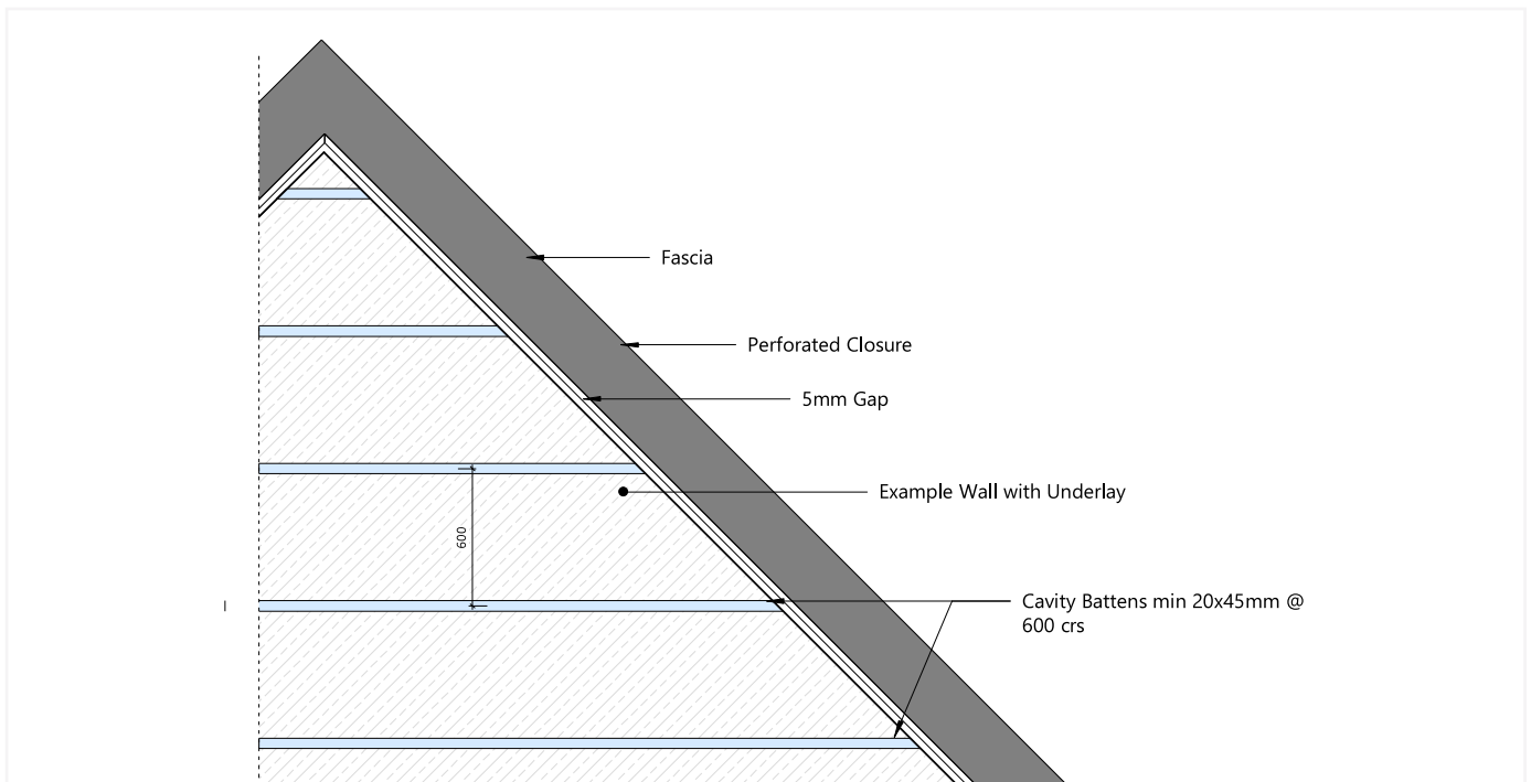
FIG 3 - BATTEN LAYOUT AROUND AN OPENING
