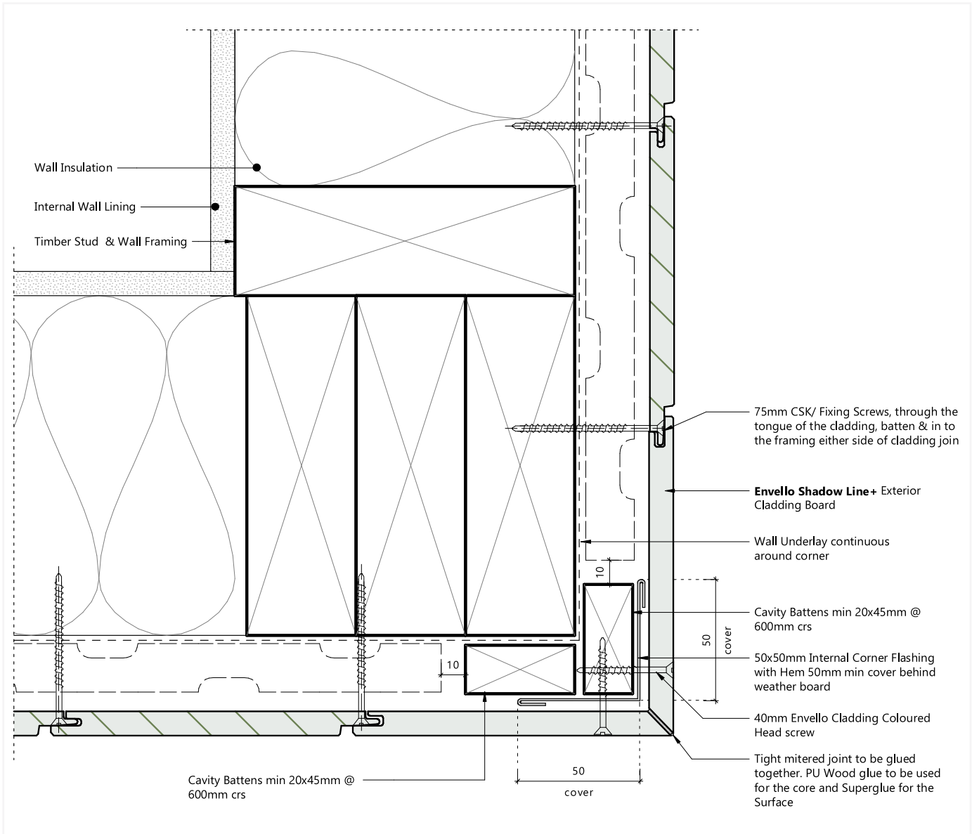
FIG. 10 - EXTERNAL CORNER PROFILE
