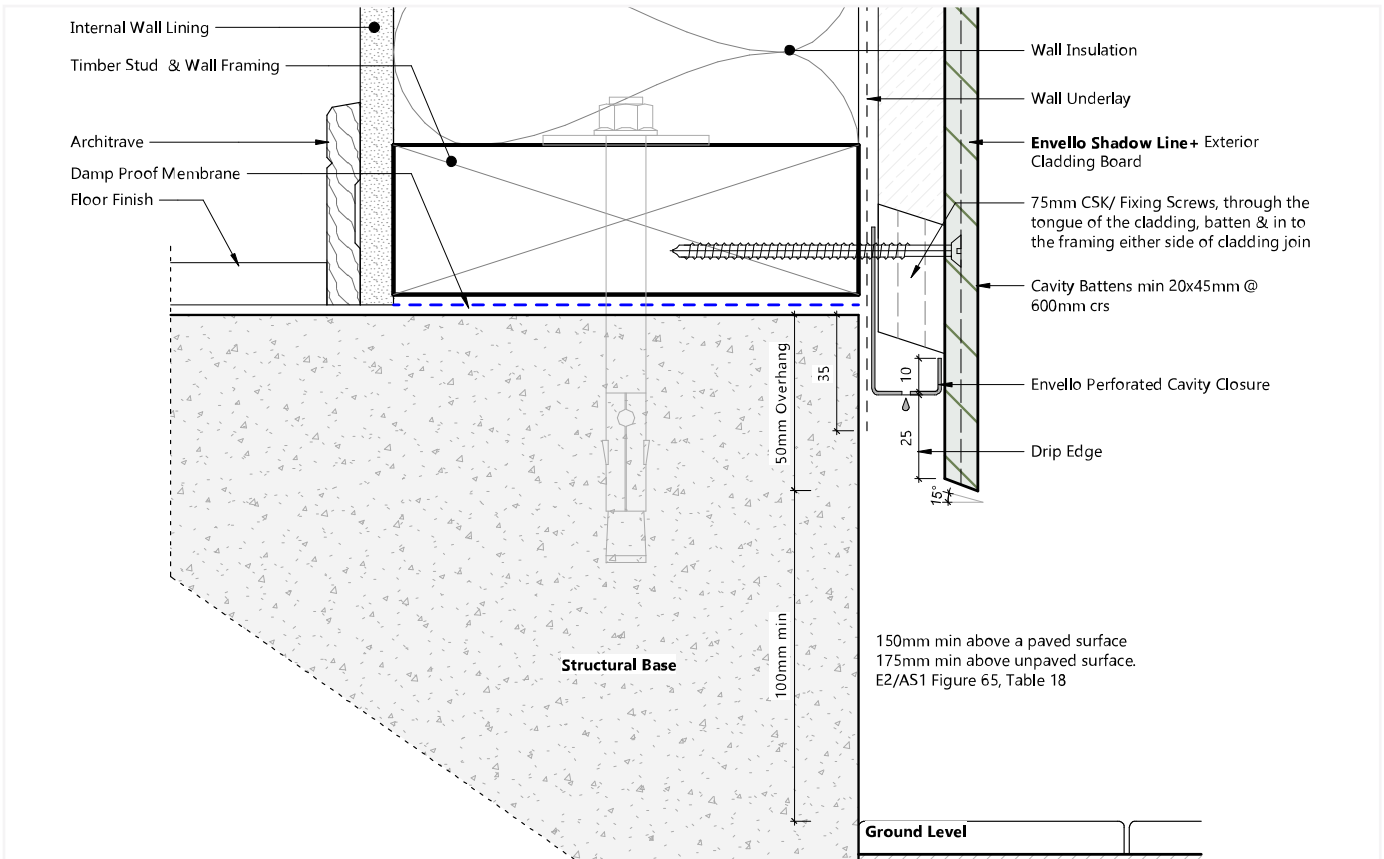
FIG. 1A - TOP & BOTTOM OF CLADDING DETAIL
