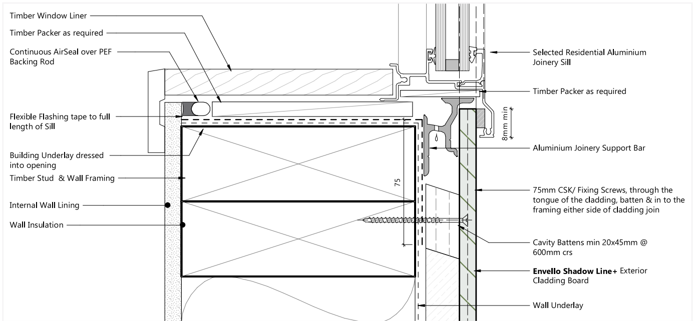
FIG. 21 - WINDOW SILL
