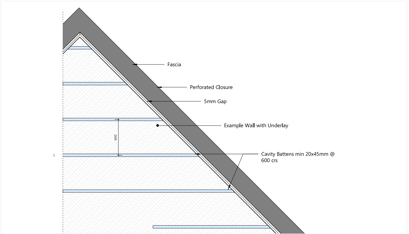
FIG 4 - BATTEN LAYOUT AT A GABLE END
