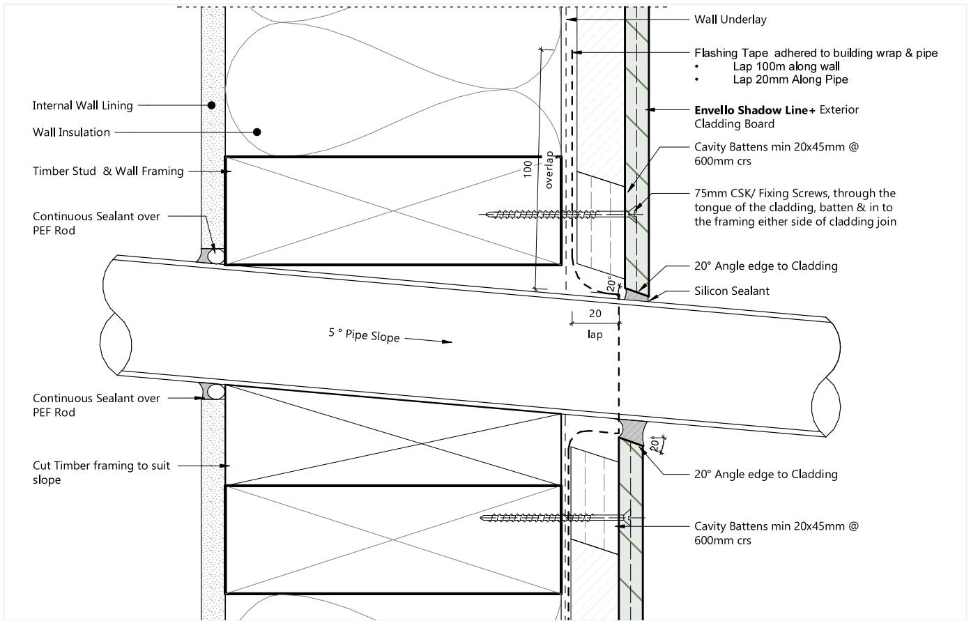
FIG. 23 - PIPE PENETRATION
