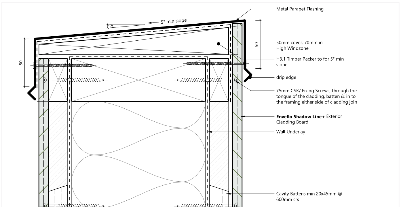
FIG. 24 - PARAPET WALL INTERFACE
