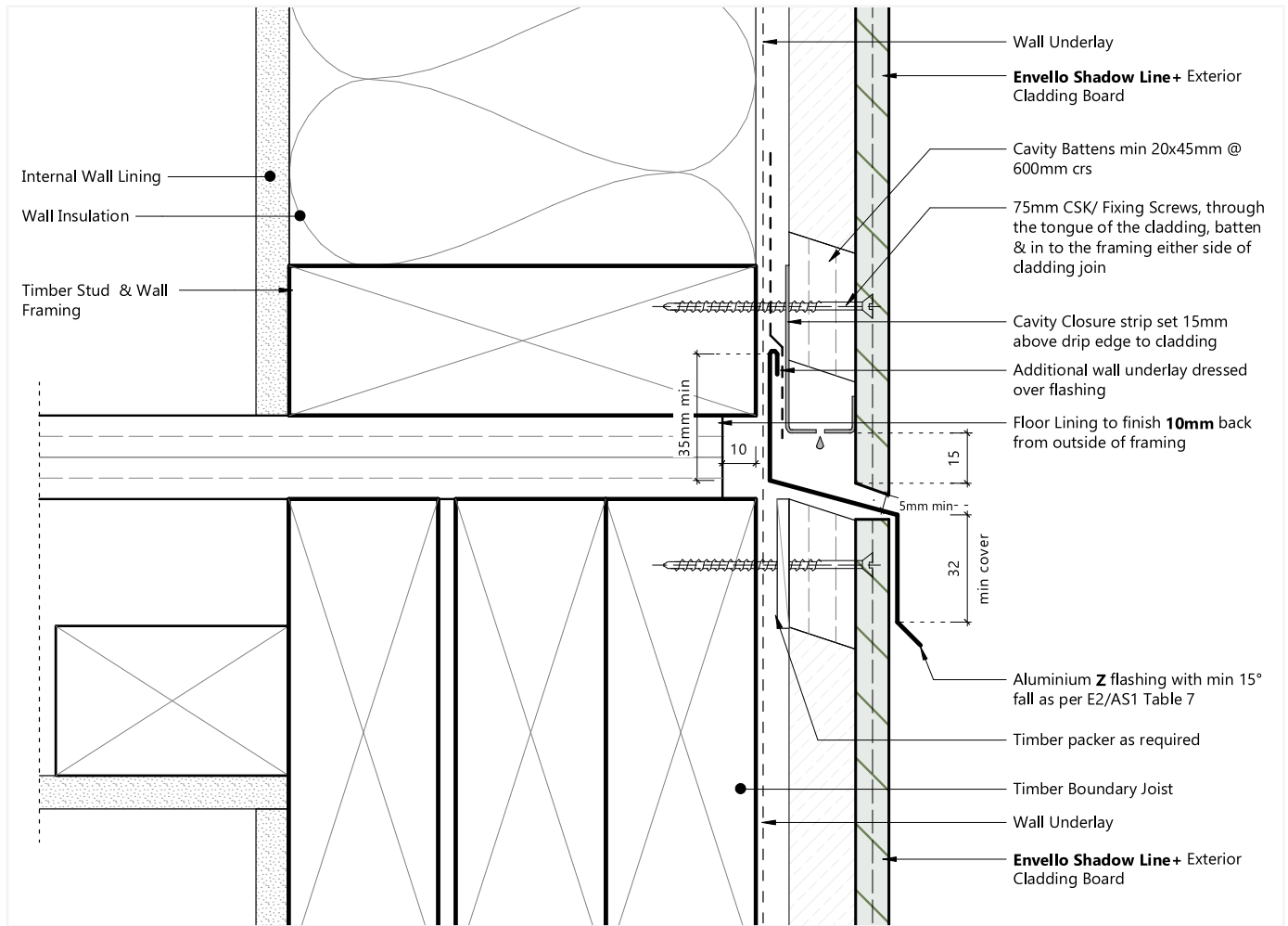
FIG. 18 - HORIZONTAL JOINT
