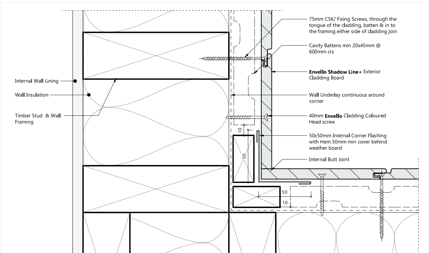
FIG. 17 - BOARD JOIN
