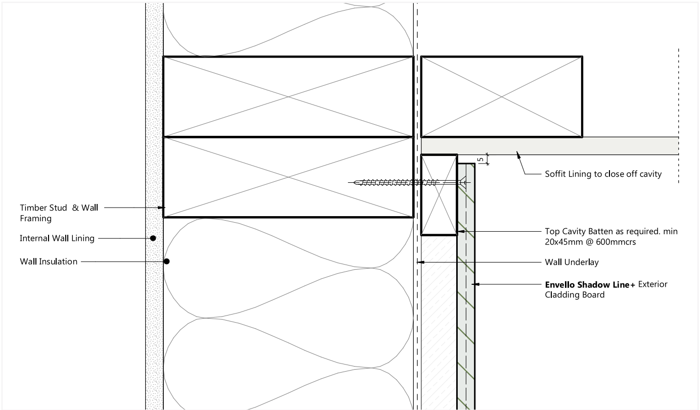
FIG. 16 - WALL HEAD
