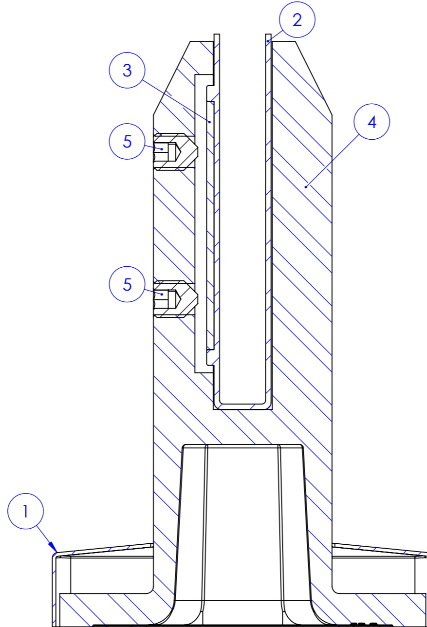
SECTION F-F
