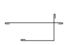
ALTERNATIVE JAMB FLASHING (OPTION 2)
