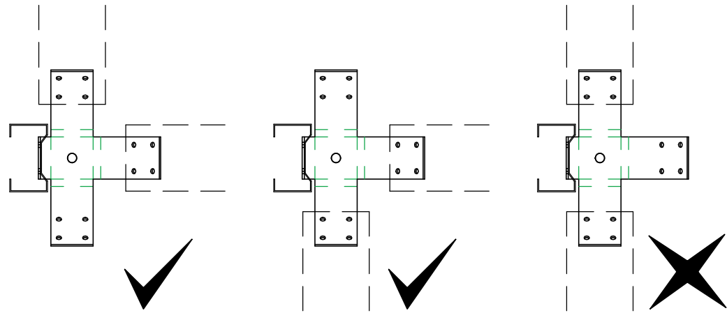
BRACE LAYOUT ARRANGEMENTS
