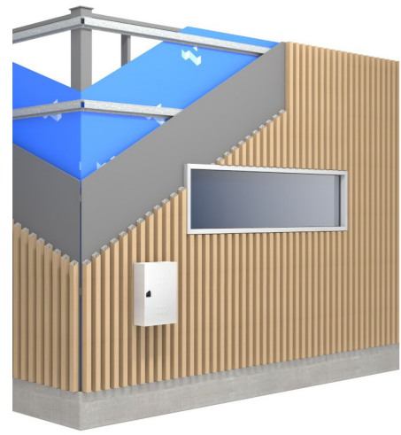
Batten - Vertical Over Exterior Cladding
