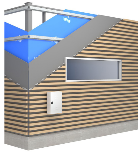
Batten - Horizontal Over Exterior Cladding
