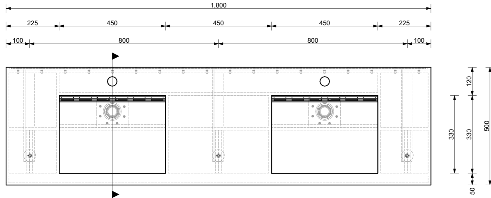
PLAN SCALE 1:10
