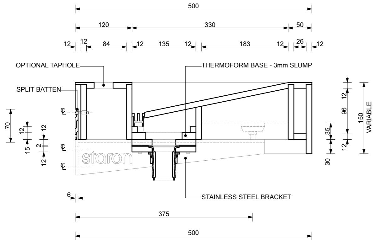
SECTION 1:5
