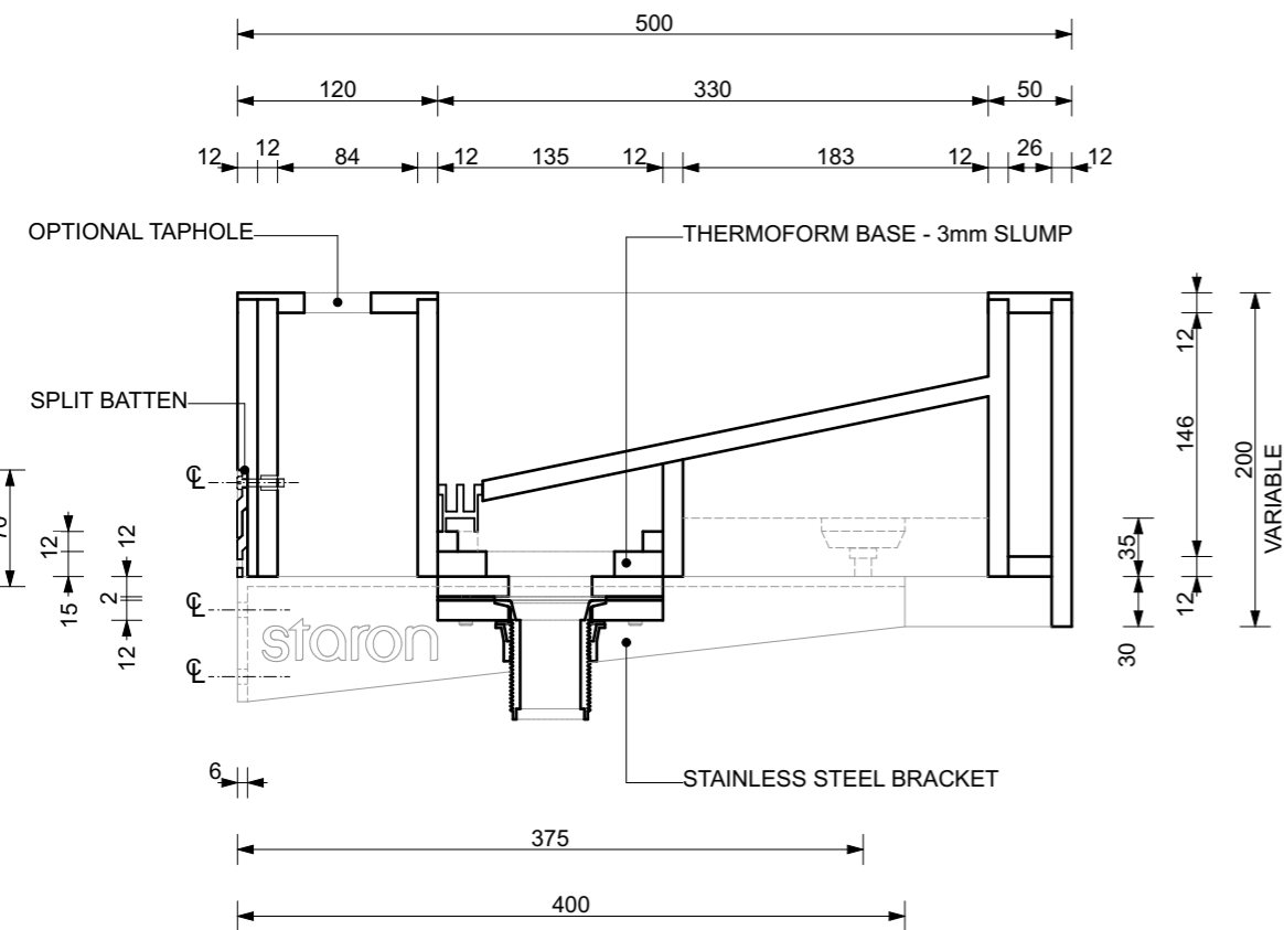
SECTION 1:5
