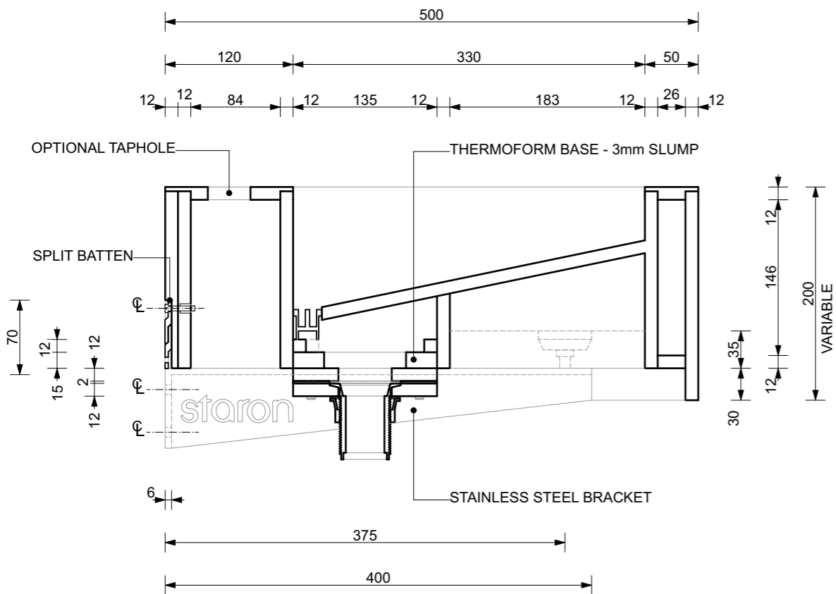
SECTION 1:5
