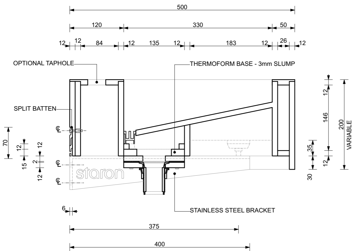
SECTION 1:5
