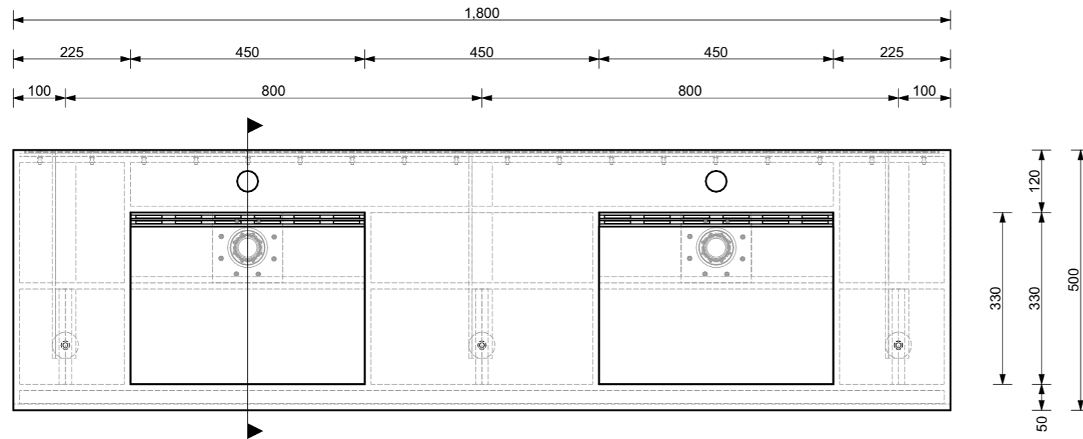
PLAN SCALE 1:10
