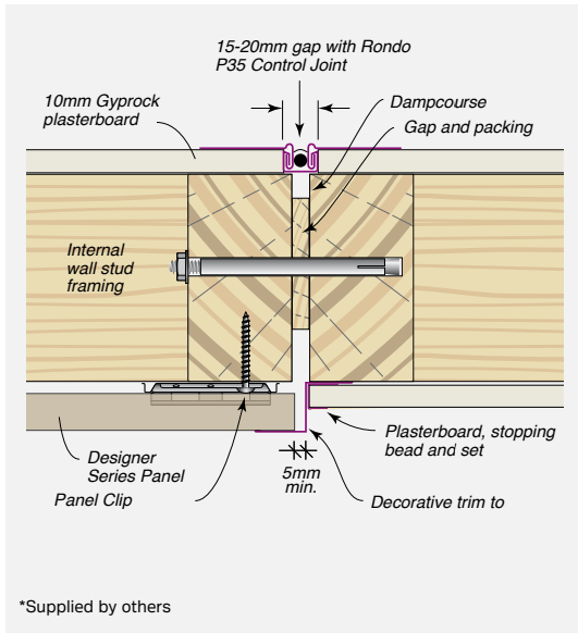
FIGURE 8.09 Typical Junction with Plasterboard Wall – Plan View
