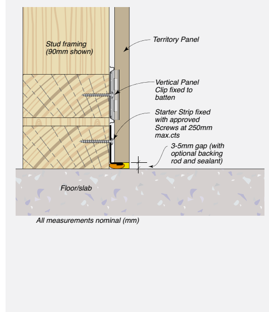
FIGURE 8.12 Base Detail - With Sealant
