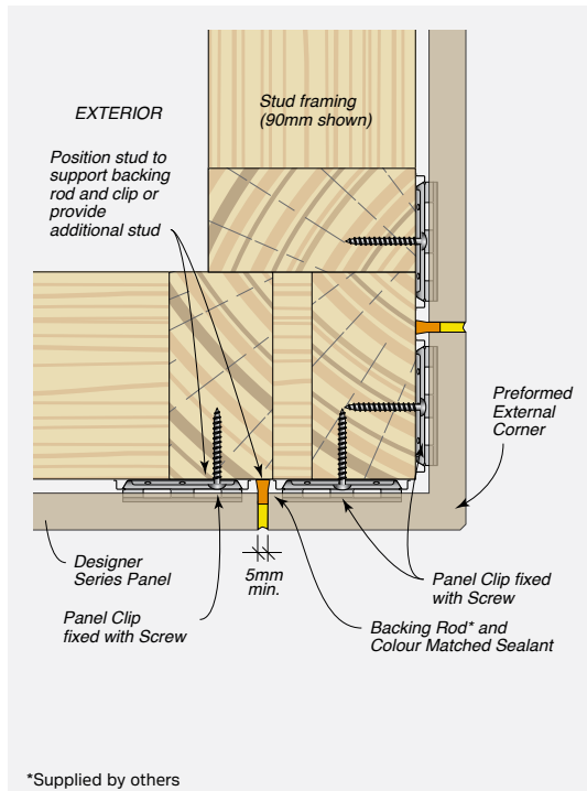
FIGURE 8.05 Preformed External Corner – Plan View
