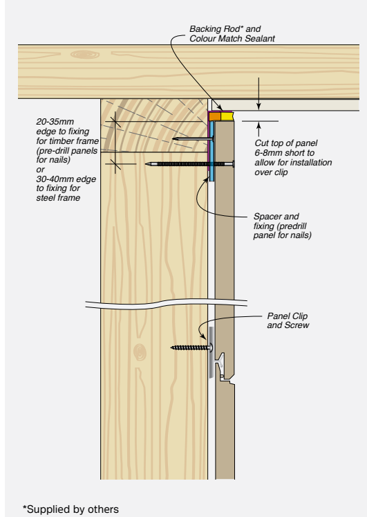
FIGURE 8.03 Head Detail - With Coloured Angle
