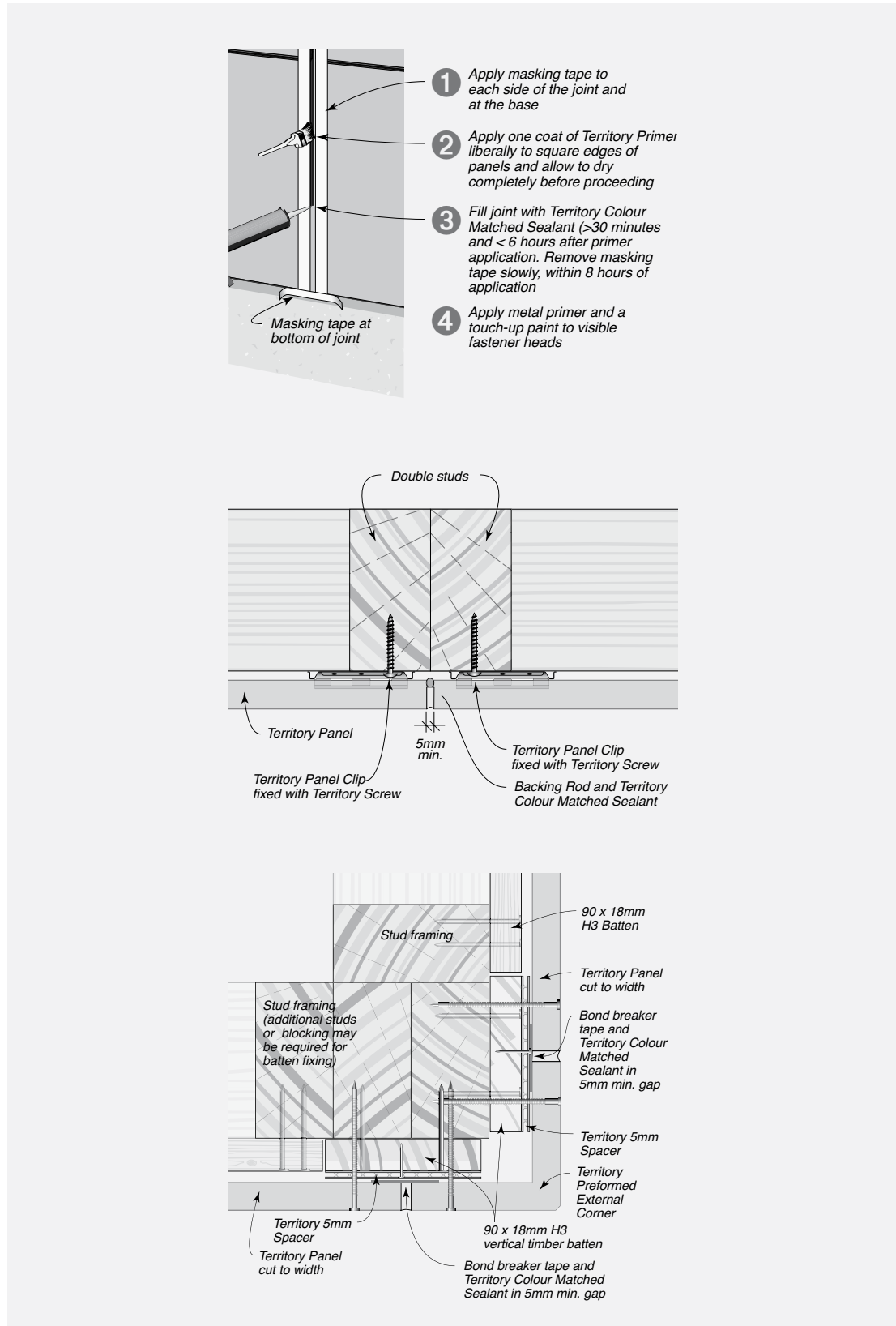
FIGURE 7.15 Typical Method for Sealing Vertical Joints
