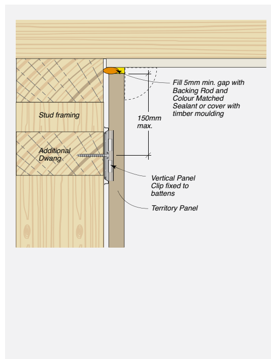
FIGURE 8.14 Head Detail - With Sealant
