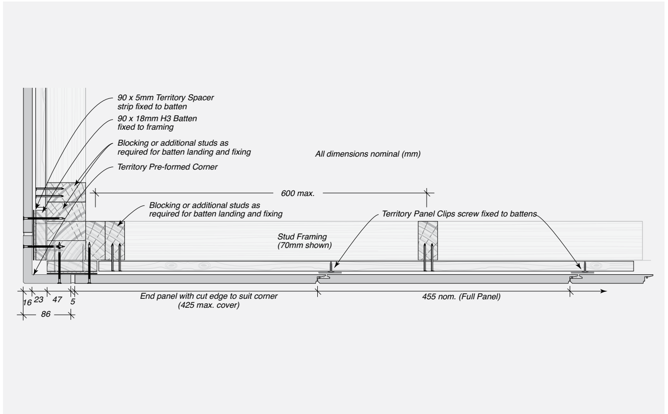
FIGURE 7.12 Typical Framing Set-Out with 70mm Timber Framing and Territory Pre-formed Corners – Plan View
