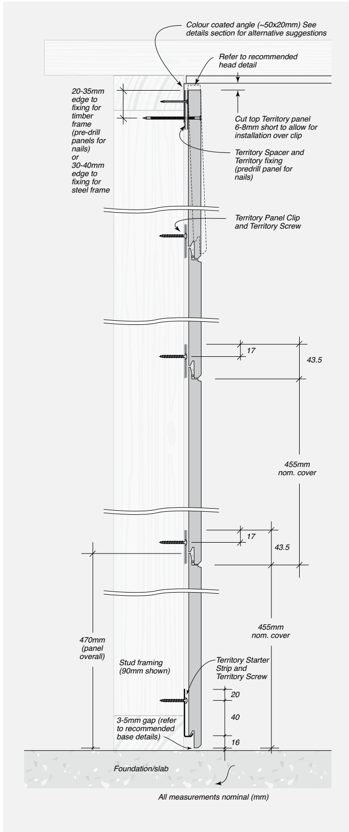
FIGURE 7.04 Typical System Cross Section - Elevation
