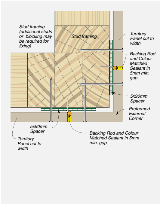
FIGURE 8.16 External Corner Detail – With Preformed Corner – Plan View
