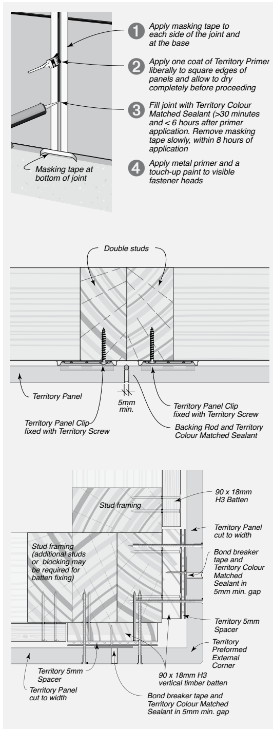
FIGURE 7.07 Typical Method for Sealing Vertical Joints
