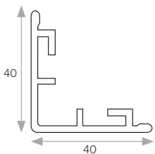
40x40mm External DRI
