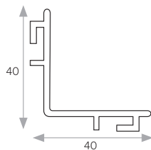
40x40mm Internal DRI
