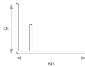
40x60mm F Mold
