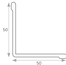
50x50mm Internal Angle
