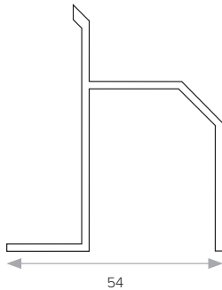
Bottom Track
