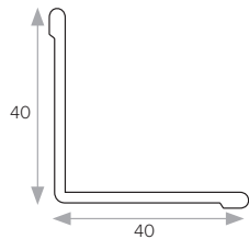
40x40mm Internal Angle
