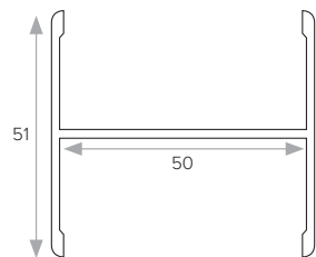
50mm I Beam
