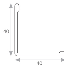
40x40mm External Angle
