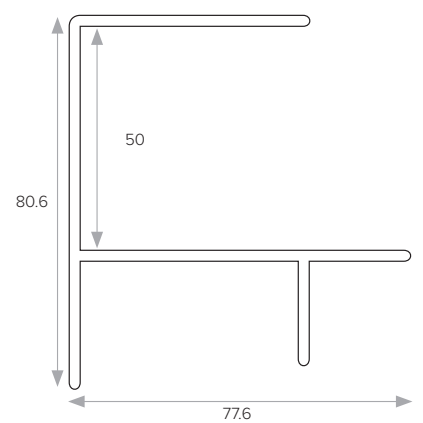
50mm Corner Connector
