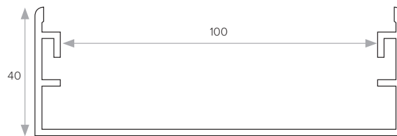
100mm DRI Channel
