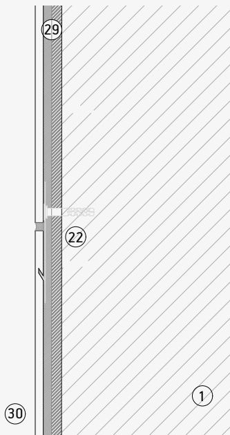
Horizontal joint
