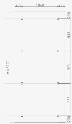
V1. Max. Design wind load: 1.5 kN/m 2
