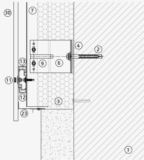
Bottom detail
