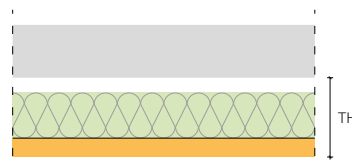
Background filling with rock wool
