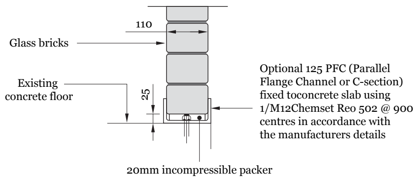
Figure 2: Lateral base restraint
