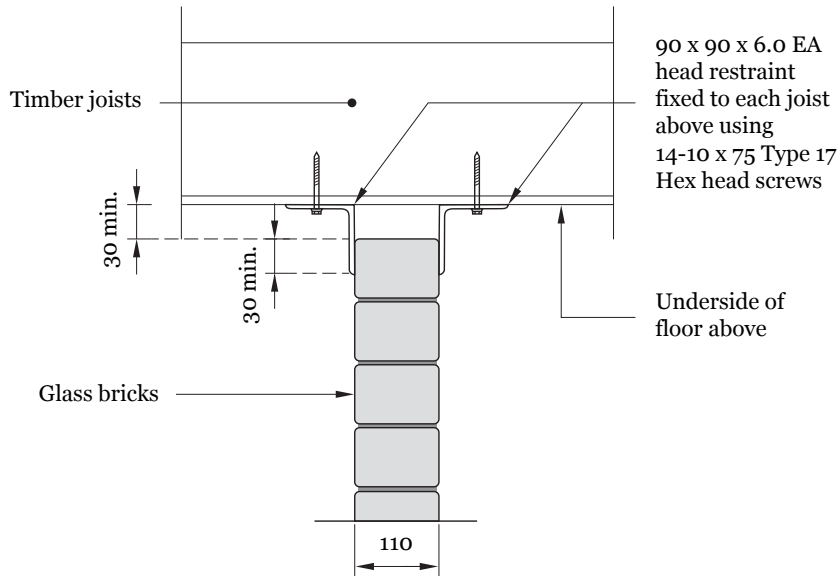
Figure 1: Lateral head restraint detail
