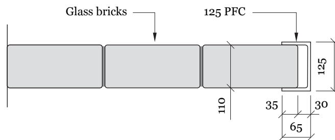
Figure 3: End detail
