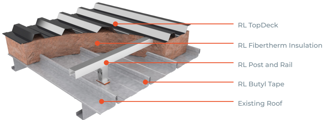
RL FiberthermX Recover System
