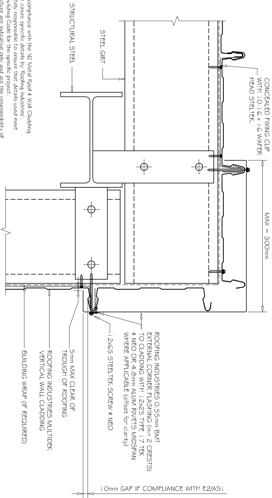
A - EXTERNAL CORNER - PLAN VIEW 1:5
