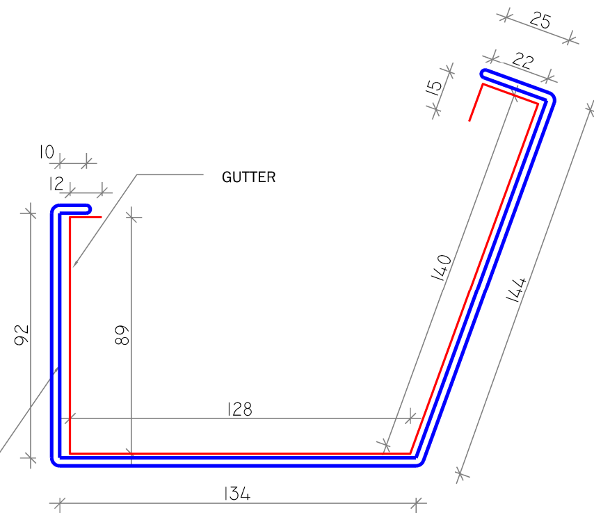
406mm CUSTOM GUTTER TYPE B
