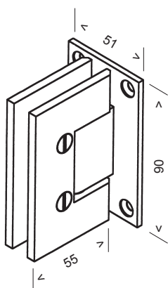
MF2 Glass to Glass Hinge
