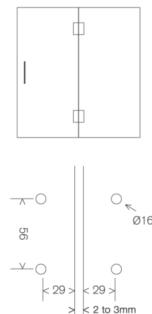
MF2-BF Glass to Glass BiFold Hinge
