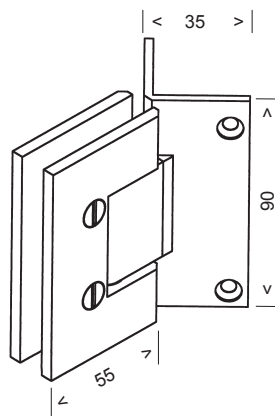
MF2-135 Glass to Glass 135° Hinge
