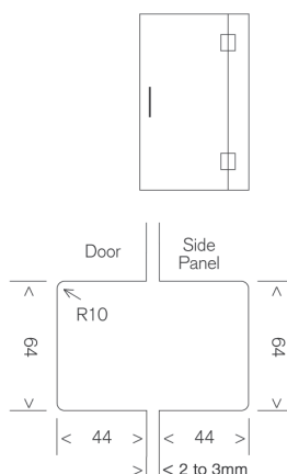
MF2 Glass to Glass Hinge
