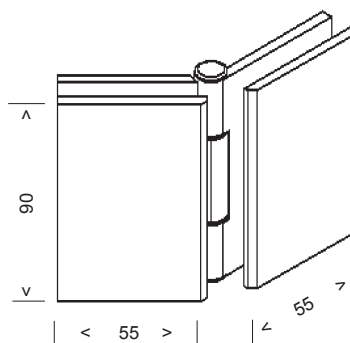
MF2-BF Glass to Glass BiFold Hinge
