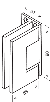
MF1-L Single Side Wall Mount Hinge
