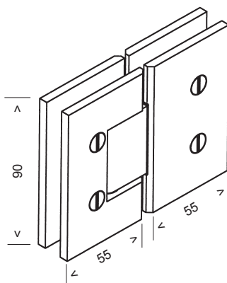
MF2-90 Glass to Glass 90° Hinge
