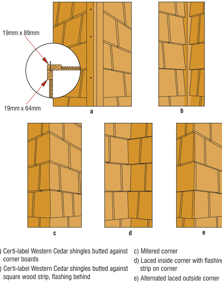
Figure 8: Corner Option Details
