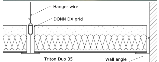
Detail: Triton Duo 35 ceiling tiles suspended on Rondo Donn DX Grid
