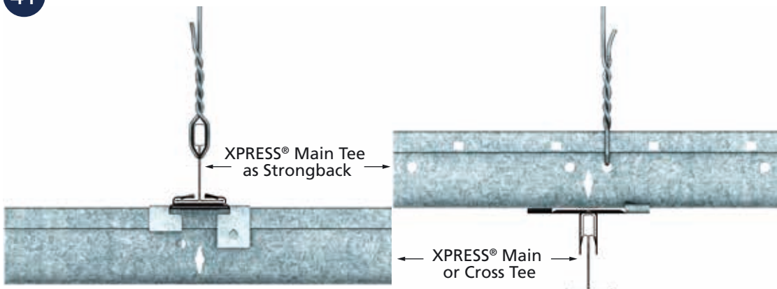
■ TYPICAL APPLICATION: STRONGBACK CLIP CONNECTION
