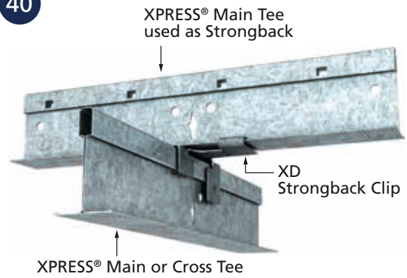
■ XD19 STRONGBACK CLIP INSTALLED
