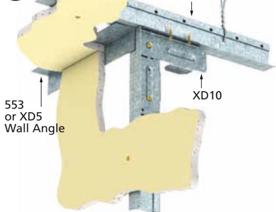
■ 90° INSIDE CORNER USING XD10
