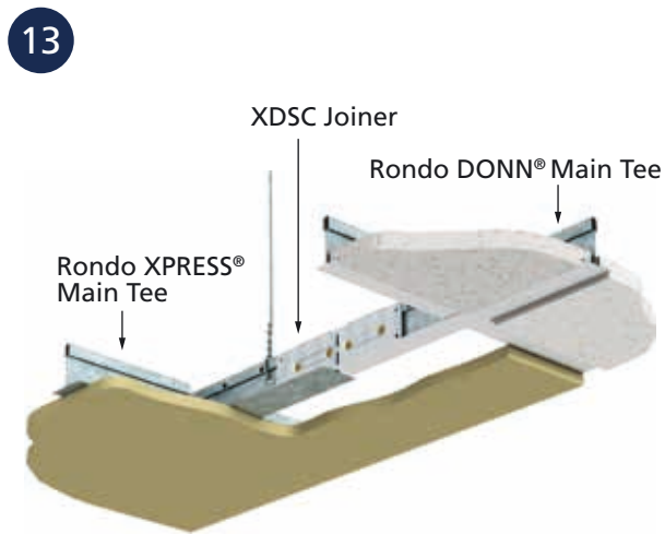
■ DRYWALL TO EXPOSED GRID TRANSITION: FIELD CUT CONNECTION
