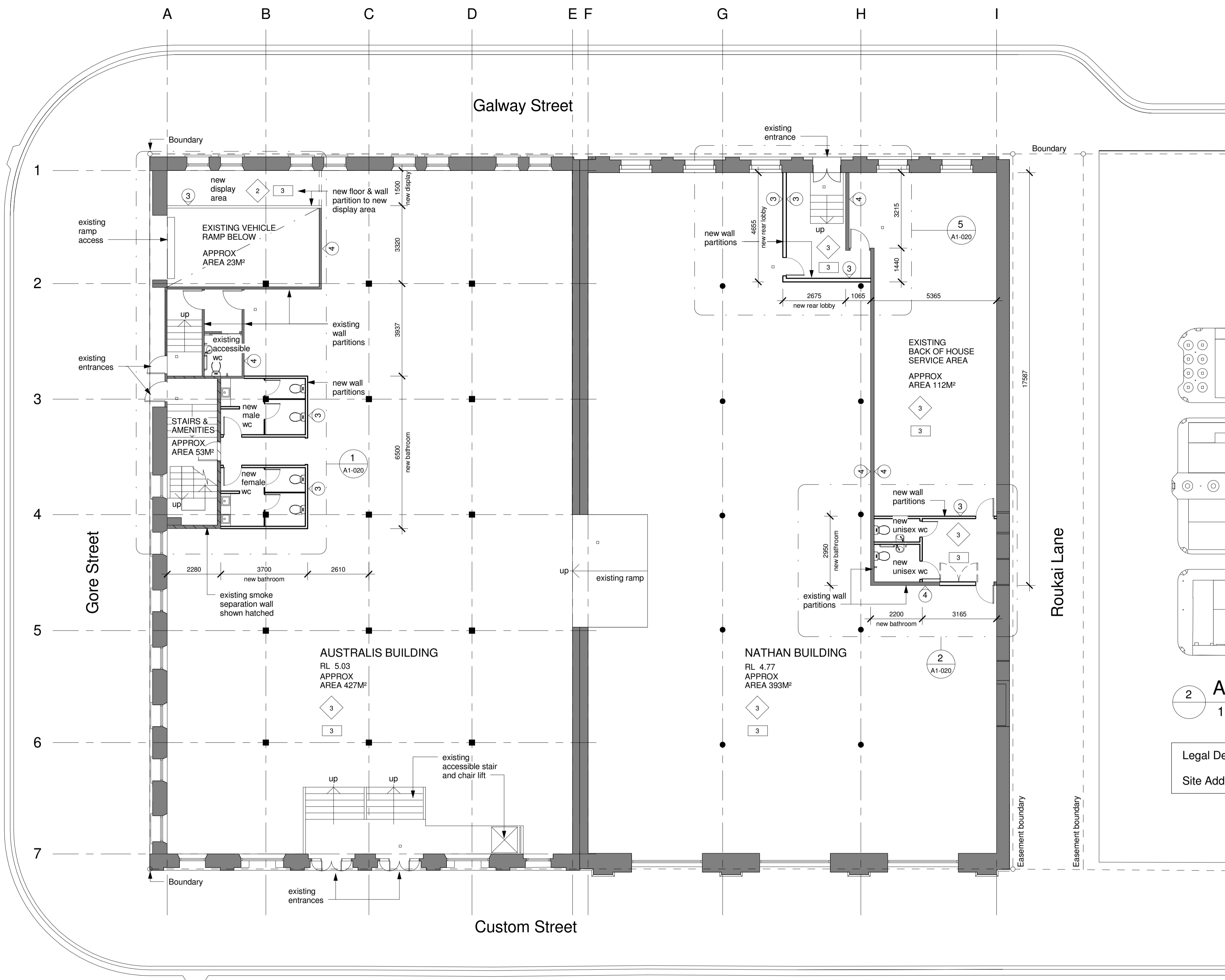
1 Ground floor - Adidas Museum / Showroom 1 : 100
